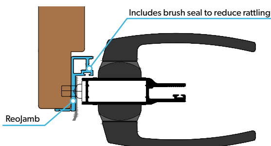
Standard Reojamb fitted to a standard timber door jamb.
