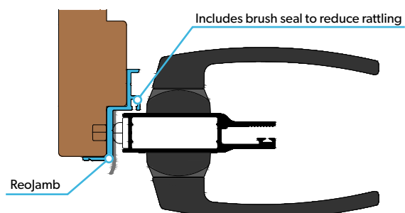
Stepped Reojamb fitted to a rebated timber door jamb.
